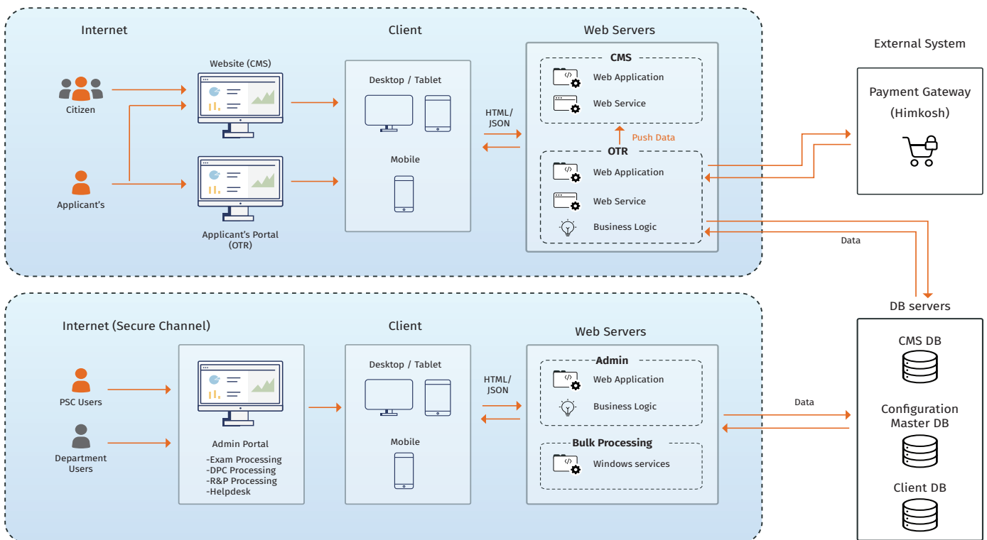
▲ PSC-Soft Deployment Architecture
