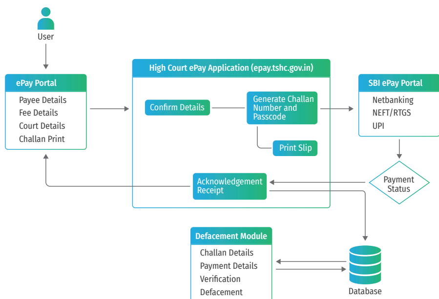
▼ Fig 9.1 : ePay Application Work Flow
