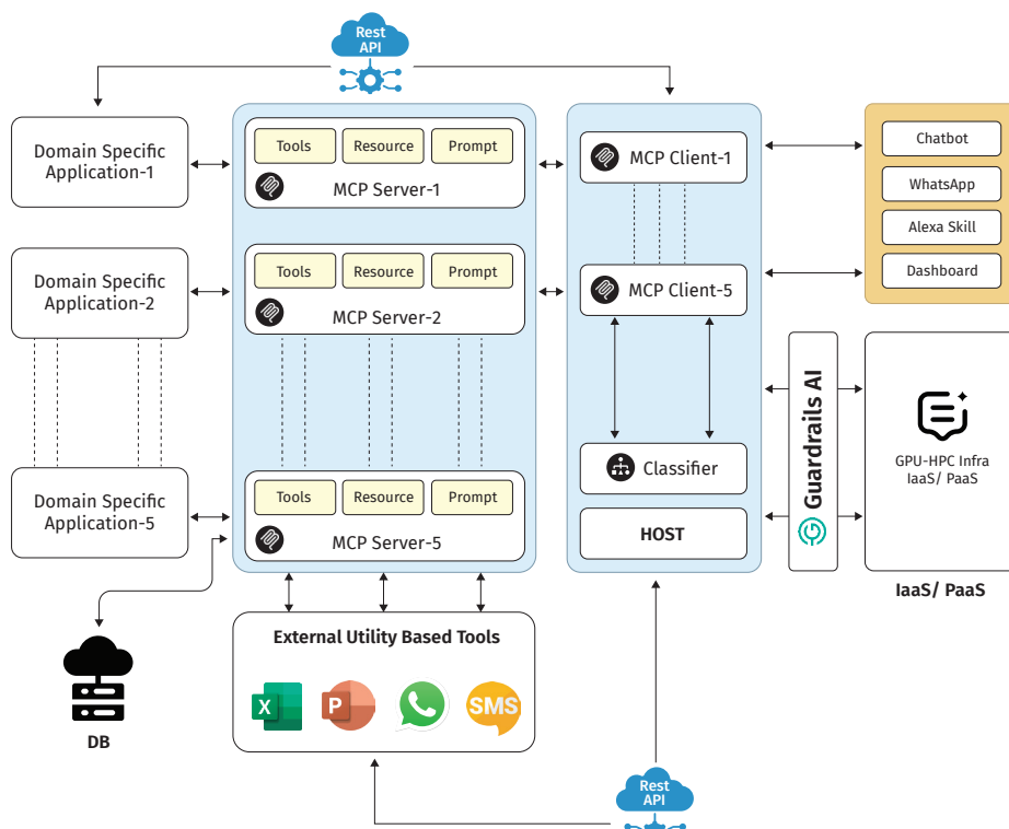
▲ Tab 11.1 MCP Architecture Overview
